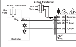
Triac Sink with Separate Transformer
