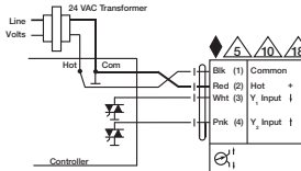
Triac Sink
