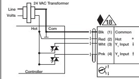
Triac Source
