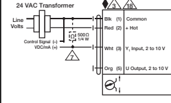
VDC / 4 to 20 mA
