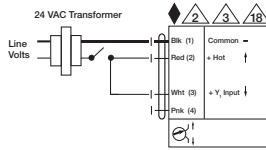
On/Off
