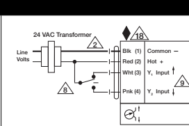
Floating Point
