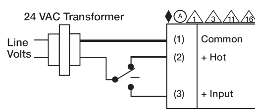
Floating Point
