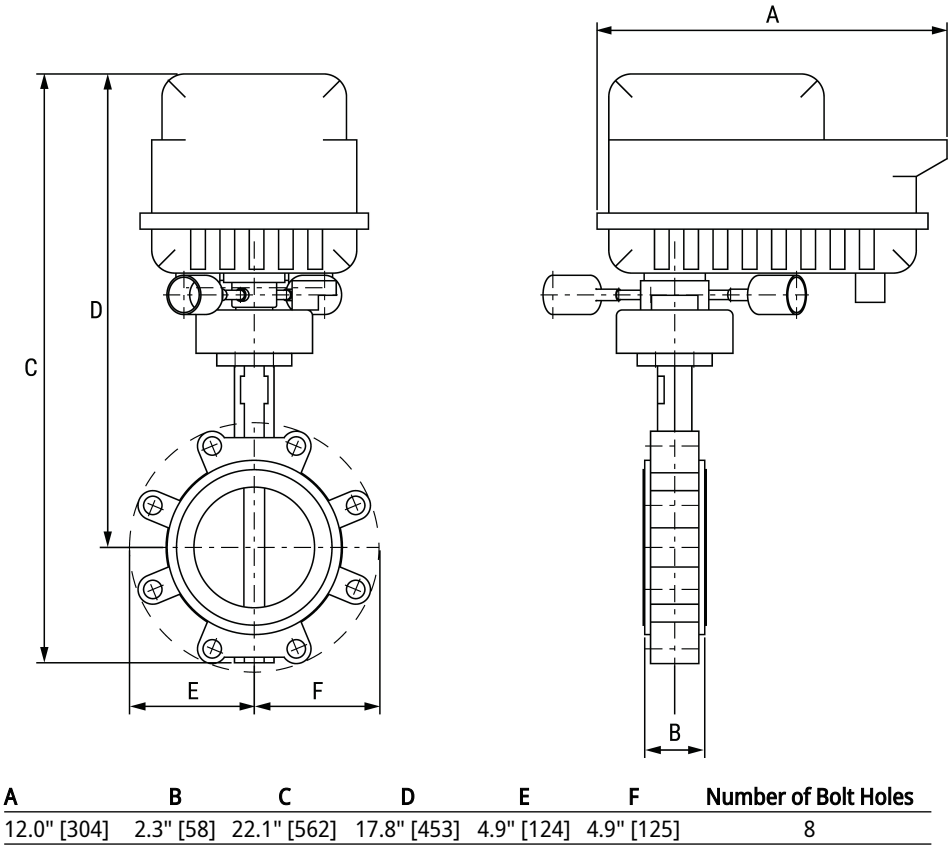
Valve with PKR Actuator
