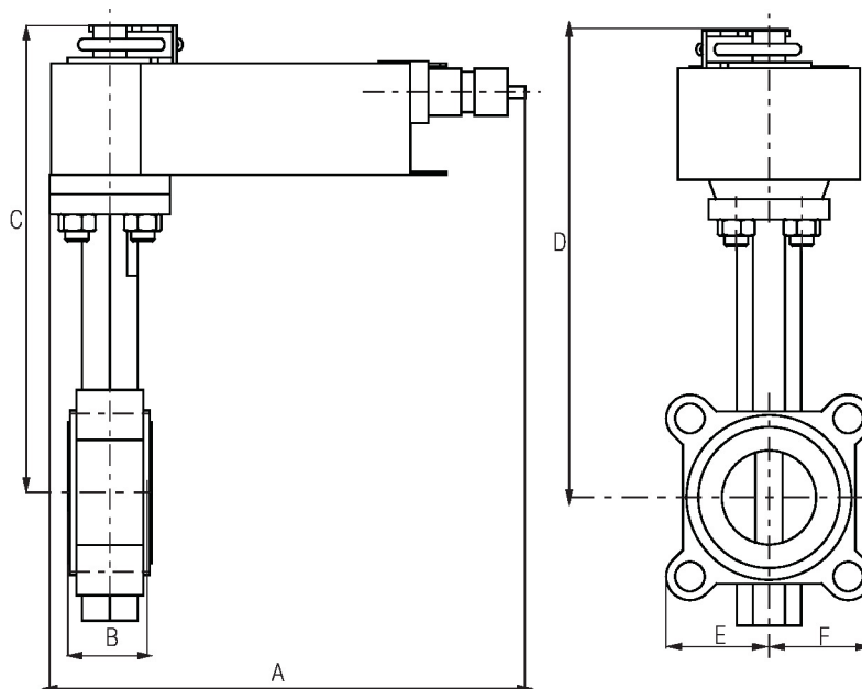
Valve with AFR Actuator
