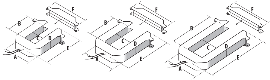
H6810/Small 200-300 Amp
